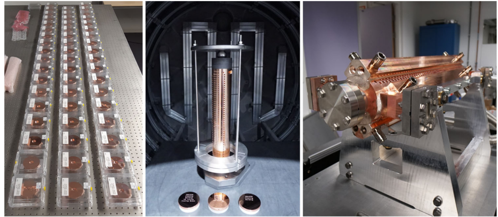
Fig. 6 Left: separate copper disks with cells and couplers inside the disks. Middle: stacked and aligned disks in the oven just before the bonding process together with 3 ‘witness disks’. Right: accelerator after complete production process
