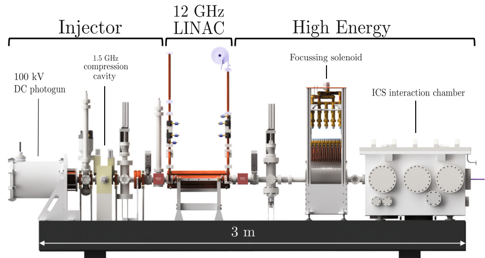
Fig. 2 Side view of the complete electron beamline including laser-electron interaction chamber. The main components of the beamline are indicated. The distance from the cathode in the DC photogun to the interaction point with the laser is 2.2 m [19]
