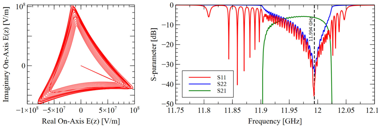
Fig. 4 Left: HFSS simulation of the real- and imaginary components of the on-axis E(z) field along the 100XS50 structure. Right: simulated S-parameters vs frequency
