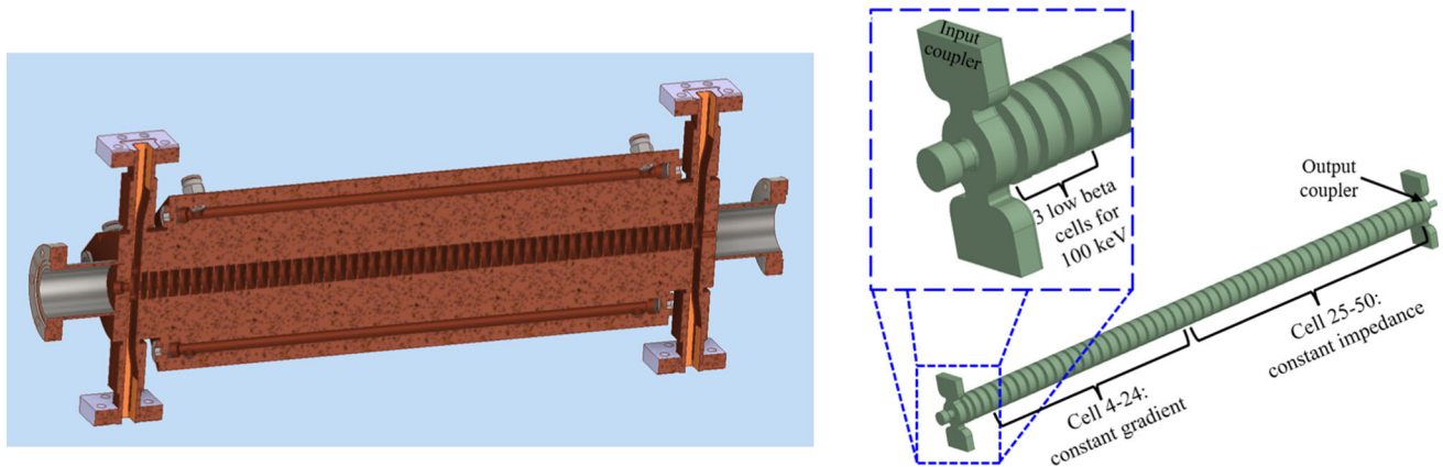
Fig. 3 Left: cross section of the mechanical design of the hybrid 100XS50 X-band structure. Right: the final inner vacuum (RF) design of the 100XS50, designed using HFSS simulations
