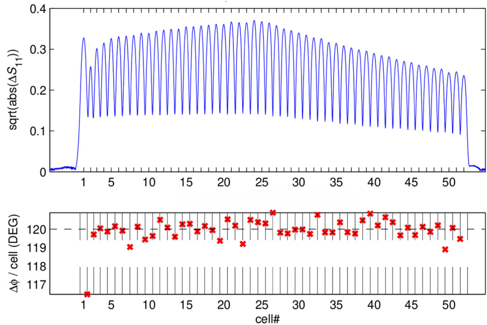
Fig. 7 Measured on-axis electric field profile (top) and phase advance between cells (bottom) after tuning, derived from bead-pull measurement of the 100XS50 structure
