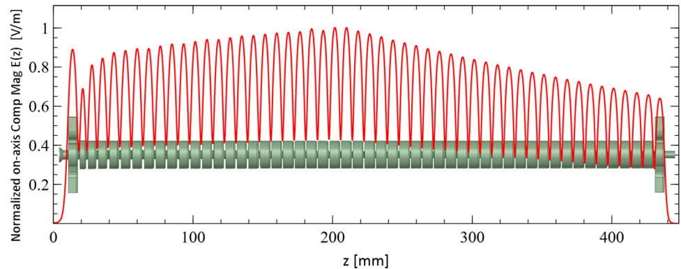
Fig. 5 HFSS simulation of the magnitude of the complex on-axis electric field along the 100XS50 structure. Cell 1–3: low beta matching cells, cell 4–24: constant gradient, cell 25–50: constant impedance
