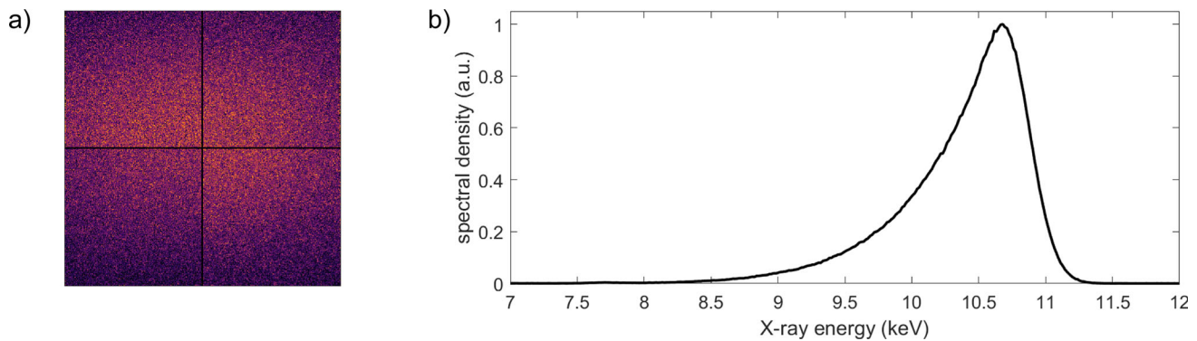
Fig. 9 Left: X-ray intensity distribution generated by ICS, measured with a 4-quadrant MediPix camera. Right: the corresponding measured x-ray spectrum. The Medipix detector was placed 1.2 m from the interaction point
